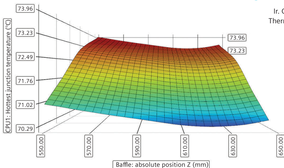
Figure 2. Response surface showing junction temperature variation with baffle position.
