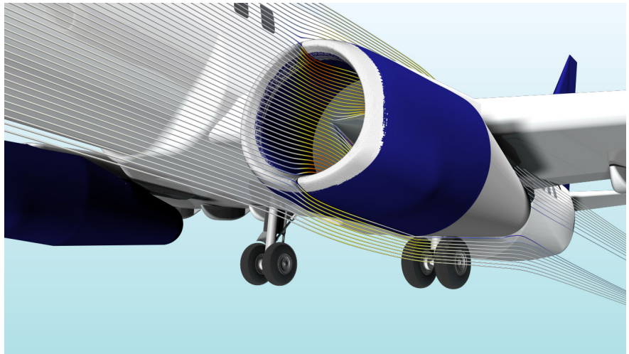
Figure 2. Predicted ice accumulation and streamlines around an engine nacelle.
