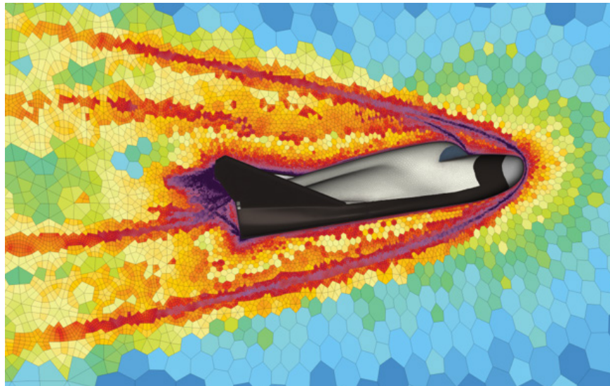
Figure 5. Adaptive mesh refinement criterion function values in Mach 10 equilibrium air model flow around the HL-20 vehicle.
