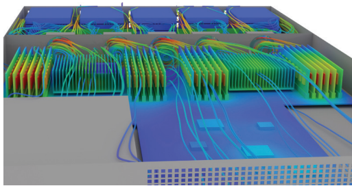
1U server with velocity colored streamlines and surface temperatures.
