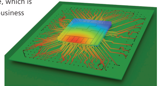
Traces on package substrate showing voltage.
