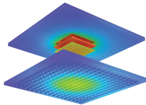
Exploded view of ball grid array package showing surface temperatures on objects.
