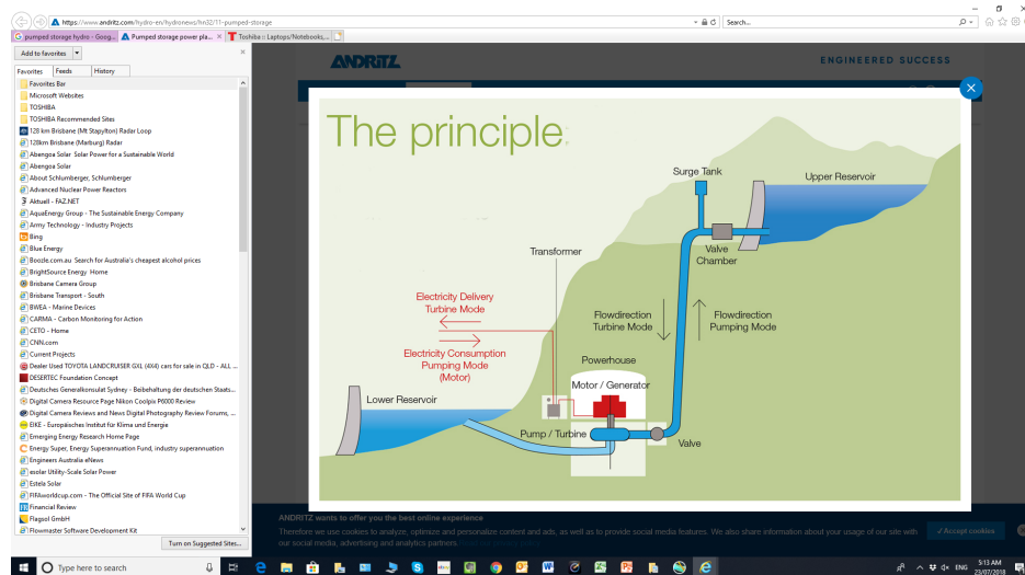
Figure 1. A typical hydro-pumped storage arrangement. (illustration courtesy of Andritz Group)
