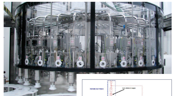
Figure 10. A Ronchi Mario filling machine and the corresponding system simulation schematic created in Simcenter Amesim.
