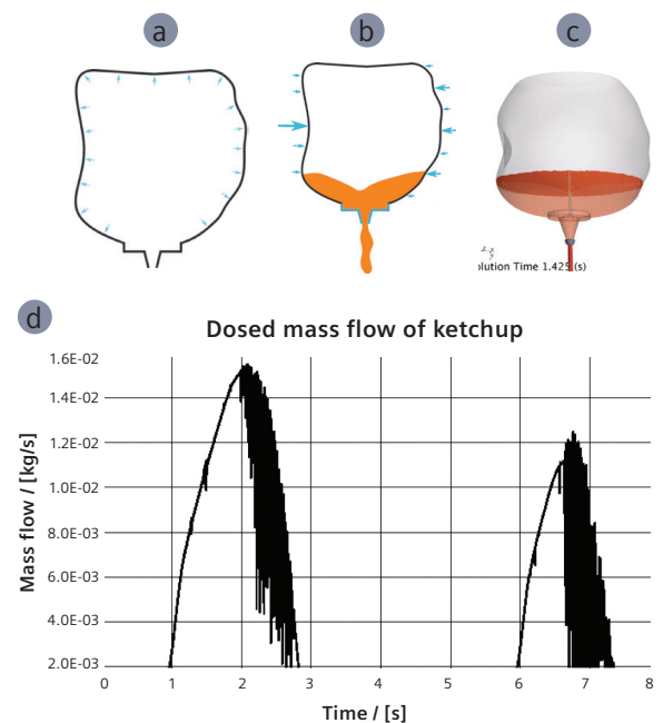
Figure 8. (a) Schematic of a ketchup bottle with simulated fingers. (b) Schematic showing flow of liquid due to squeezing of the bottle. (c) CFD simulation showing dispensing of ketchup. (d) Dosage of ketchup.
