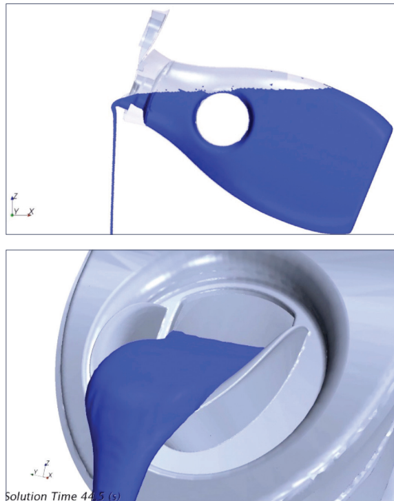
Figure 7. Simcenter STAR-CCM+ simulation showing the pouring process from a typical laundry detergent pack with a close-up of the nozzle design.
