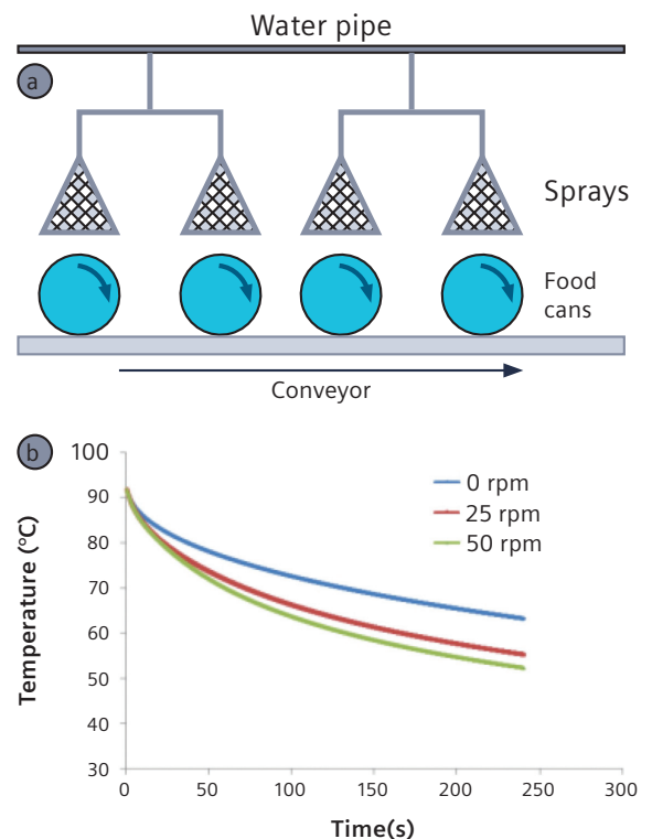
Figure 6. (a) The spray cooling system showing rotating cans on a conveyor. (b) Effect of rotation rate on cooling of cans calculated using CFD simulation of spray and heat transfer with Simcenter STAR-CCM+.
